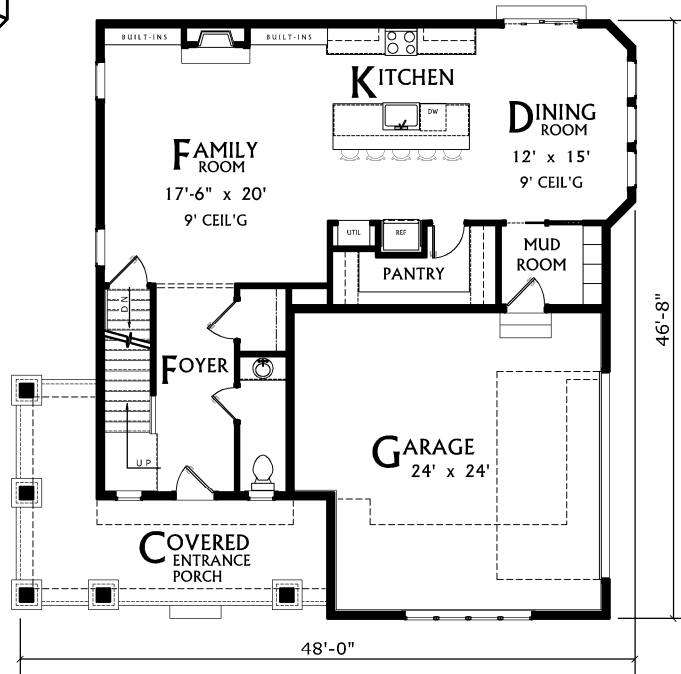
MAIN LEVEL
